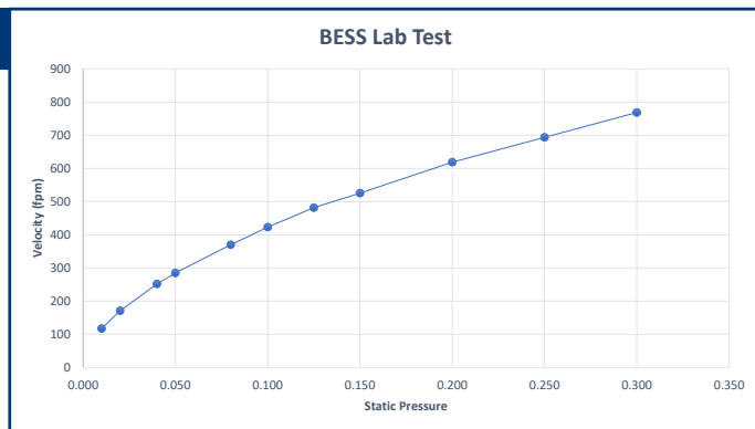
BESS Lab performance test using 6" (45/15) Munters Celdek evaporative pad and Dandy Brown-Out light trap.
