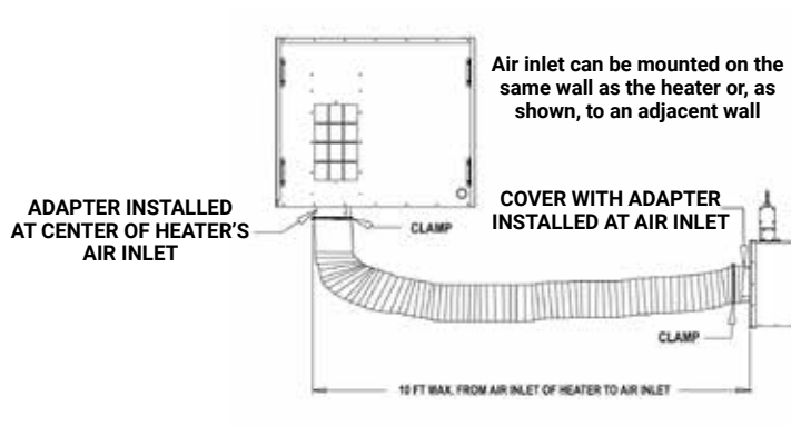
Indoor Mount with Air Inlet Transition Kit
