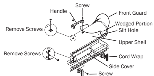
Figure 4 - Handle and Cord Wrap Installation
