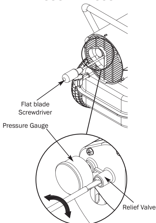
Figure 22 – Adjusting Pump Pressure
