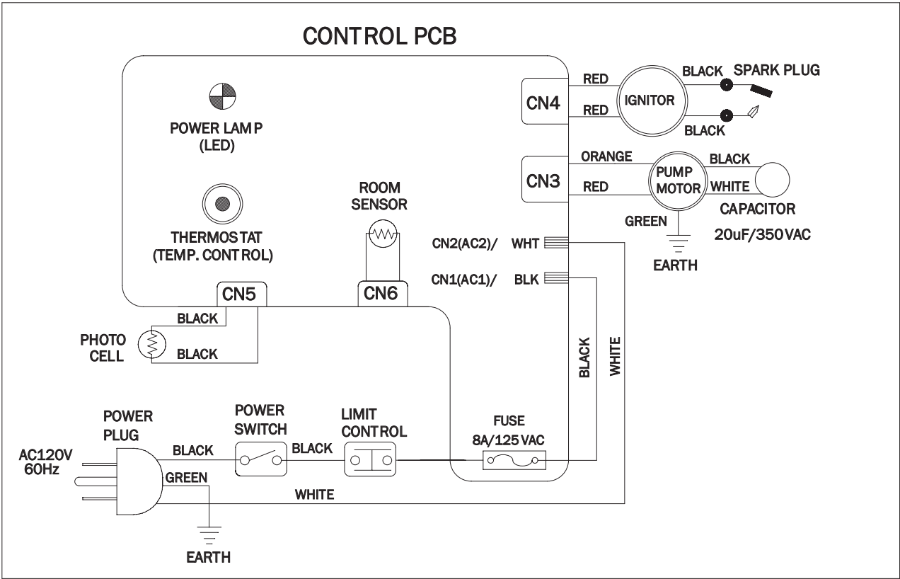
Figure 26 - Wiring Diagram Models CP125FK, CP175FK, CP220AK
