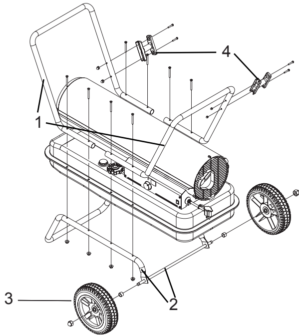
Figure 30- Repair Parts Illustration for Models CP125FK, CP175FK, CP220AK
