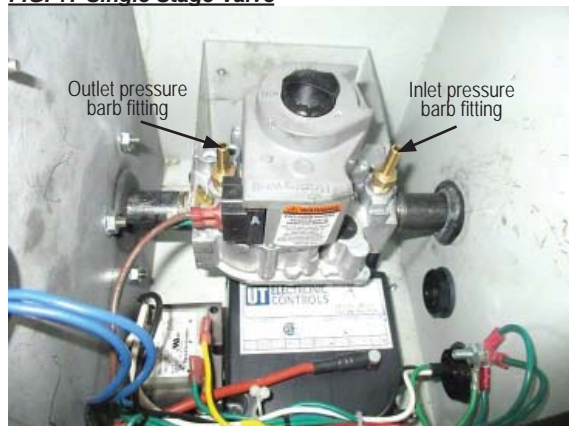
FIG. 17 Single Stage Valve
